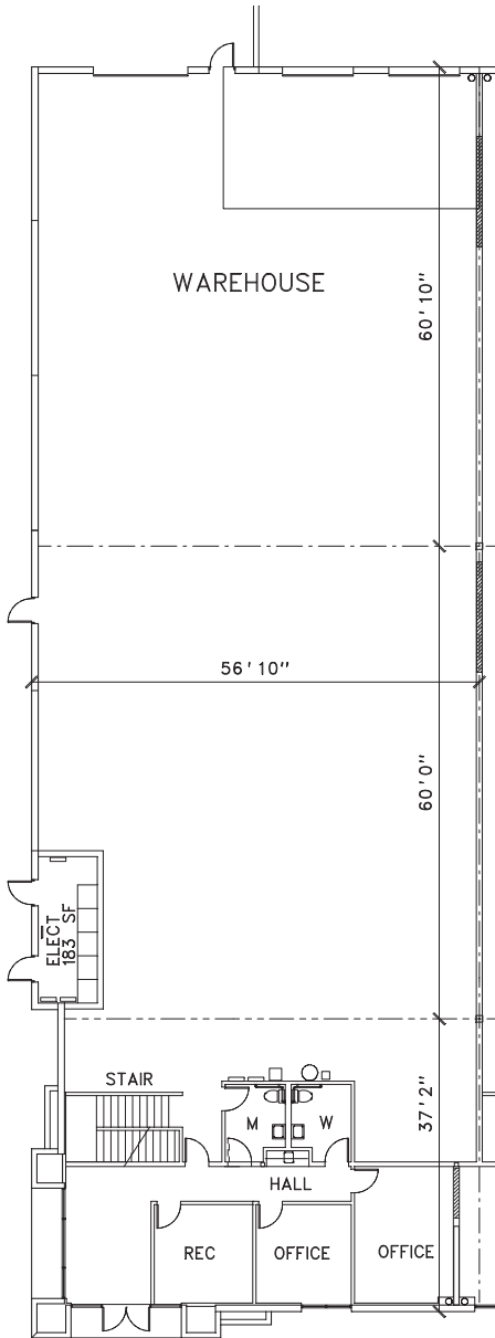
First Floor
